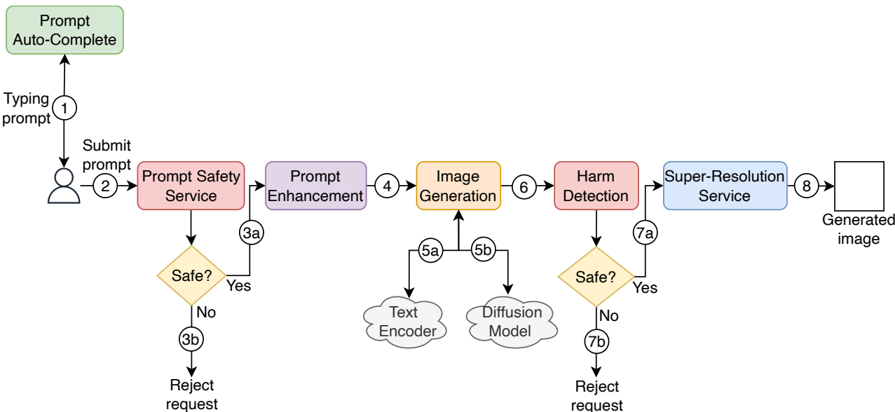
Figure 20: Inference pipeline
