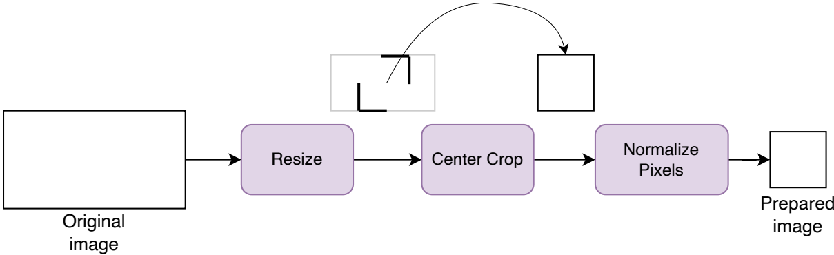
Figure 6: Image preparation steps
