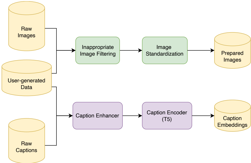
Figure 18: Data pipeline
