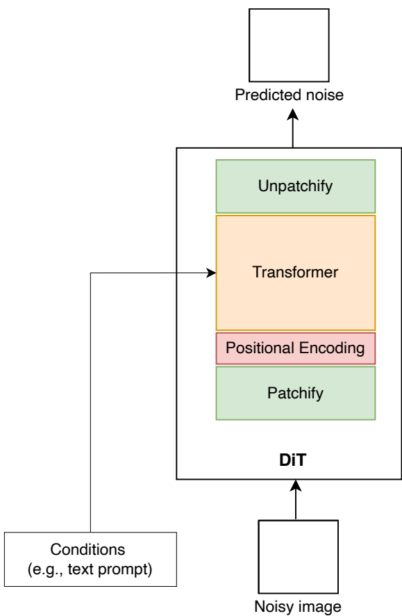
Figure 11: DiT components
