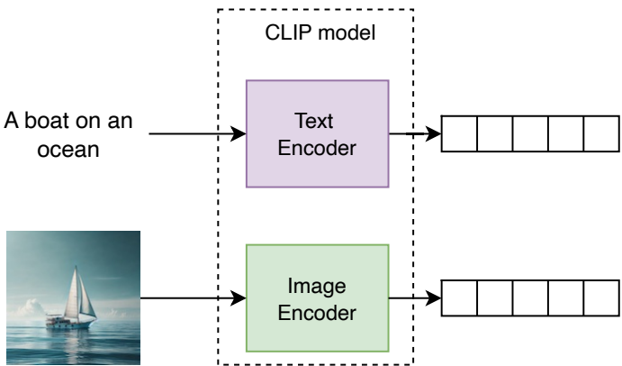
Figure 16: CLIP encoders
