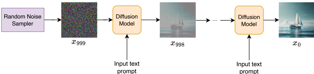
Figure 15: Sampling process
