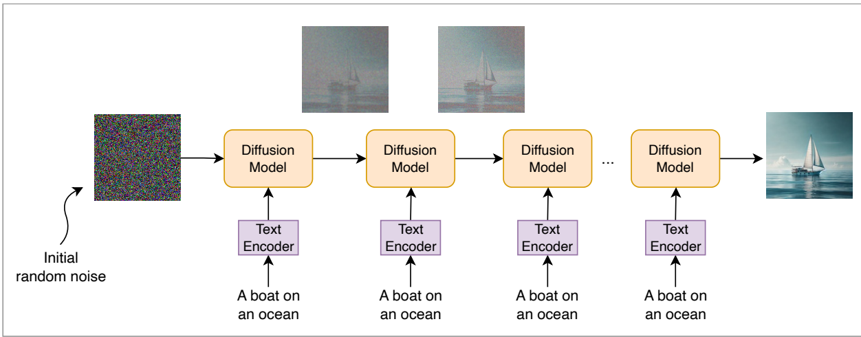
Figure 4: Diffusion-based text-to-image generation
