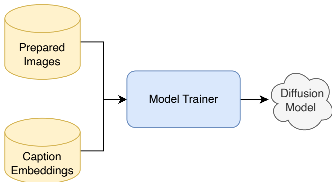
Figure 19: Training pipeline
